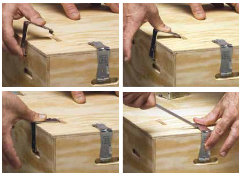
Assembly with a reusable locking system of tabs and slots
